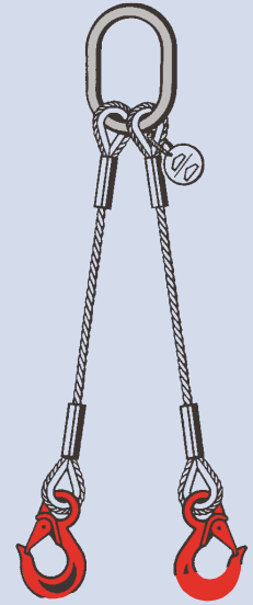
1219. 2-leg wire rope sling with safety hook
