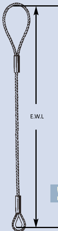
1170. Wire rope sling with pressed loop and pressed thimble
