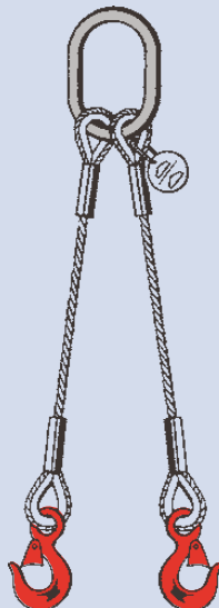
1215. 2-leg wire rope sling with safety eye hook
